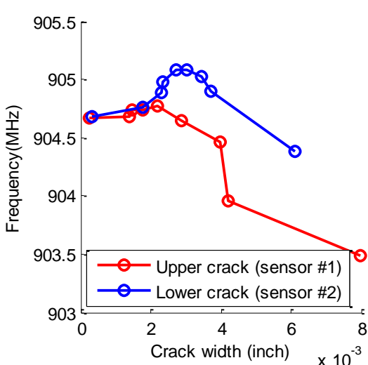
(c) Resonance frequency versus crack width
