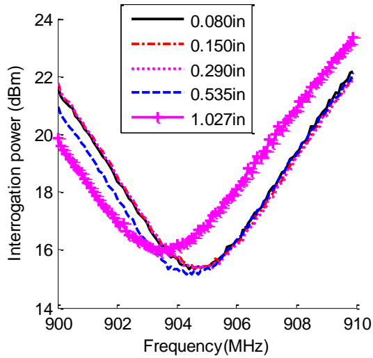
(a) Average interrogation power from antenna sensor #1
