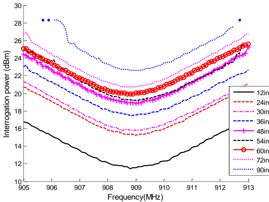
Fig. 10. Interrogation power at different interrogation distances
