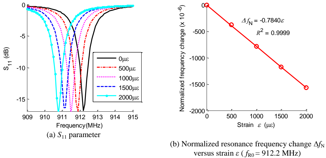
Fig. 4. Strain simulation results of the passive slotted antenna sensor from COMSOL
