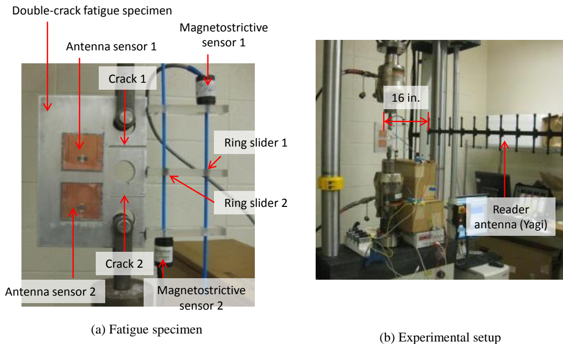
Fig. 11. Experimental setup for the fatigue test of passive slotted-patch antenna sensor
