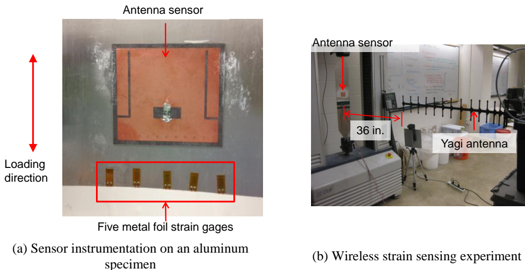
Fig. 5. Experimental setup for a tensile test with 36 in. interrogation distance
