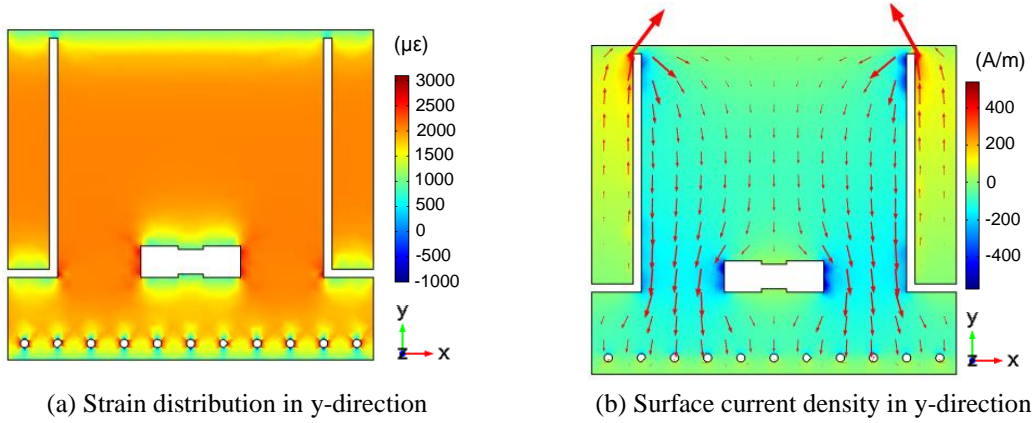
Fig. 3. Field distributions from mechanics-electromagnetics coupled simulation
