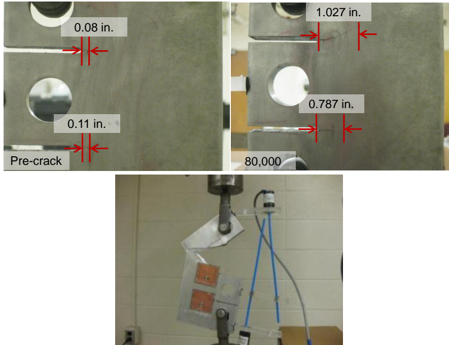
Fig. 12. Photos of double-crack specimen at different crack lengths
