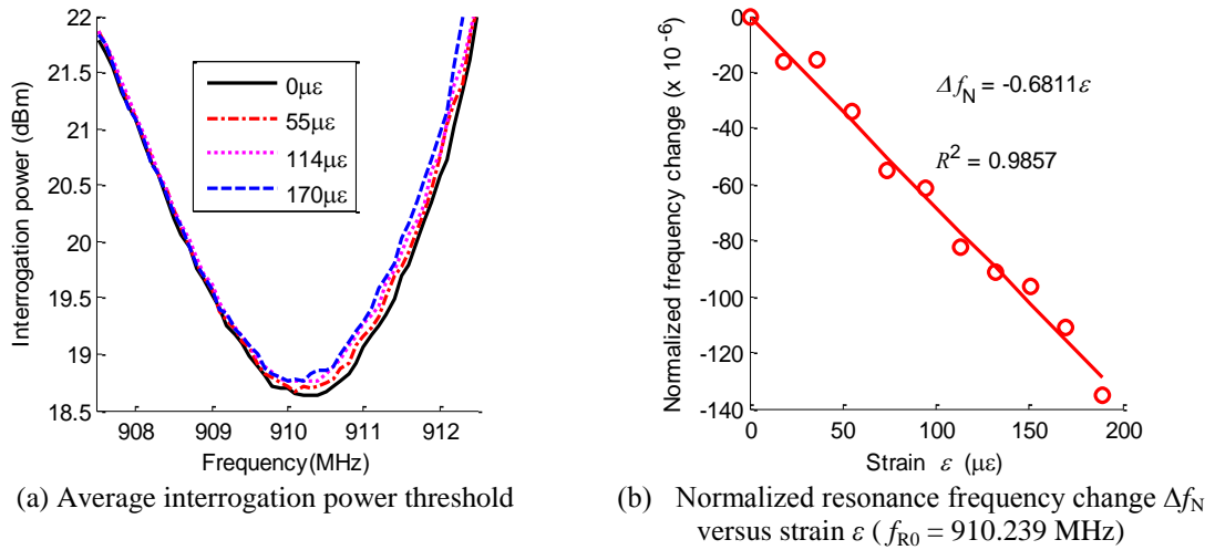
Fig. 6. Tensile testing results at 36 in. interrogation distance
