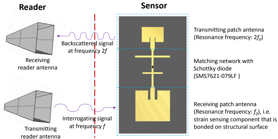
Fig. 1. Operation mechanism of a frequency doubling antenna sensor system
