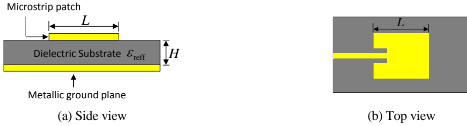
Fig. 2. Microstrip patch antenna
