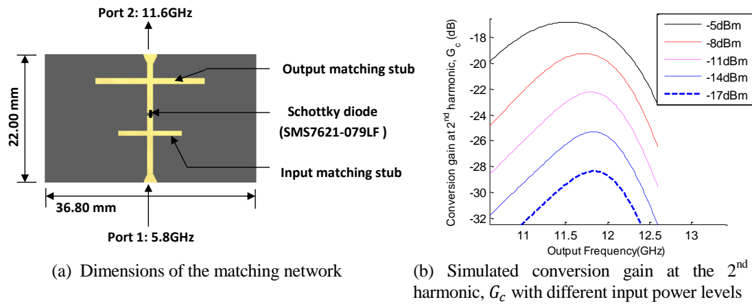
Fig. 5. Matching network design
