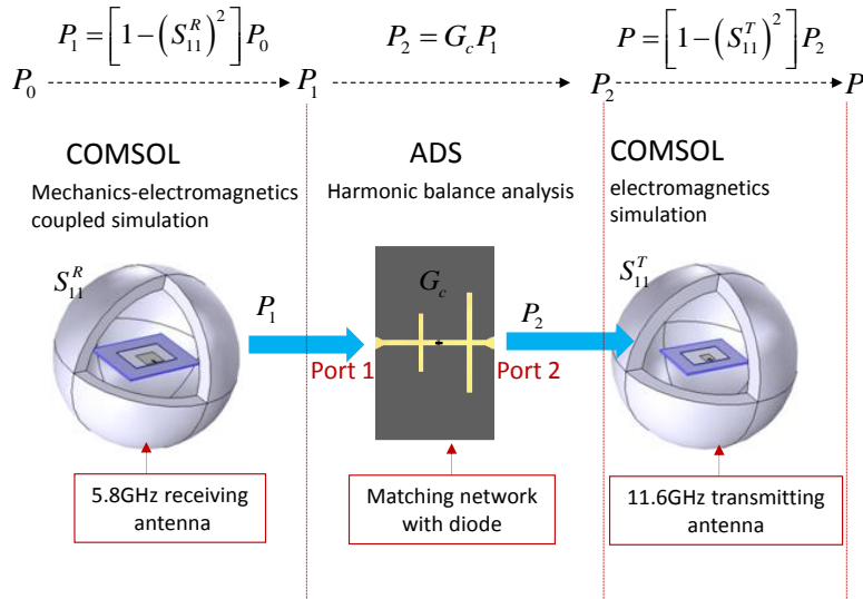
Fig. 7. Flow chart illustration of the multi-physics coupled simulation for the entire sensor
