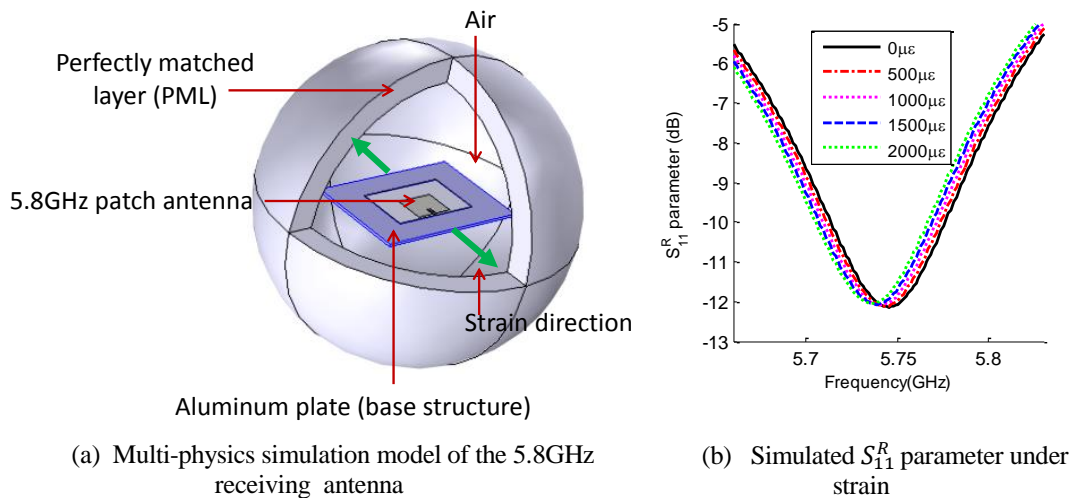
Fig. 6. Multi-physics modeling and simulation for the receiving (5.8GHz) patch antenna
