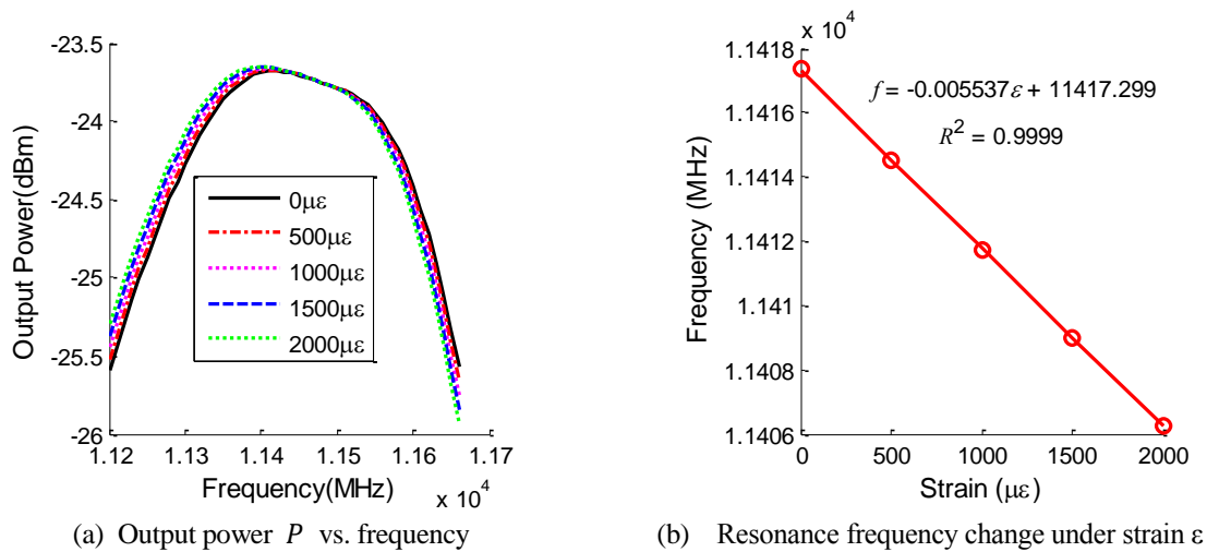
Fig. 8. Multi-physics simulation result
