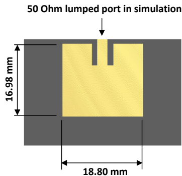
(a) Dimensions of the 5.8GHz receiving antenna
