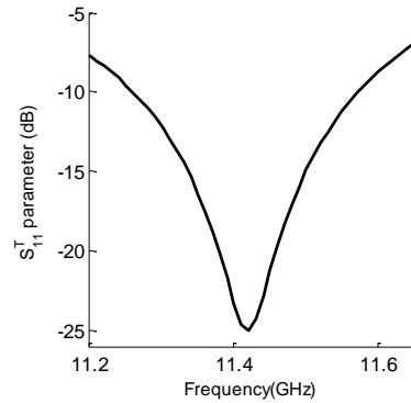
(b) Simulated S_{11}^T parameter
